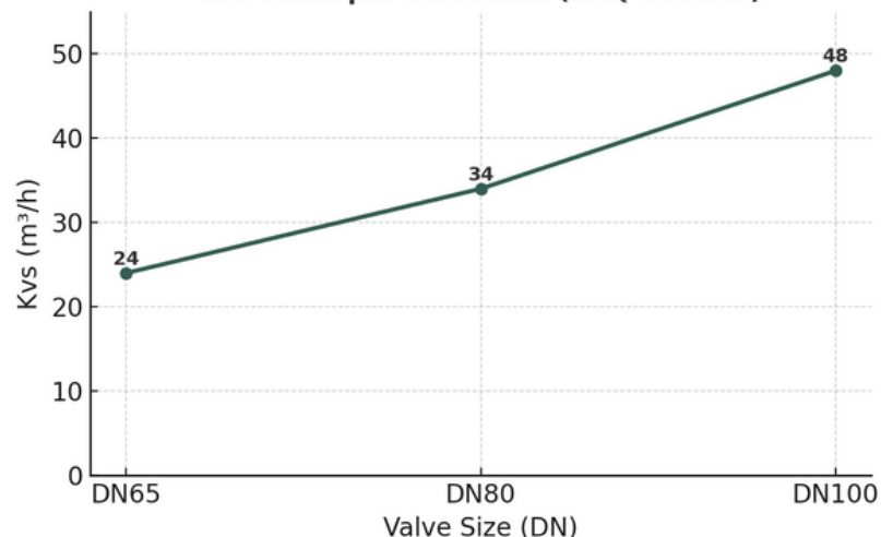
Kvs Value per Valve Size (BRQ-9000HF)
